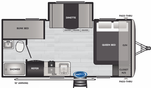
1760BH | WEIGHT 3796 | LENGTH 21' 5"
