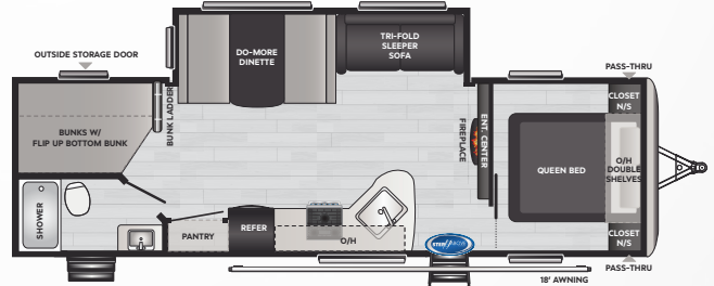
282BH | WEIGHT 6907 | LENGTH 32' 2"
