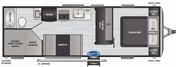
260BH | WEIGHT 5311 | LENGTH 28' 10"
