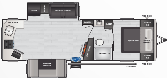
NEW! 281RK | WEIGHT 7411 | LENGTH 32' 5"
