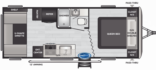
202RD | WEIGHT 4780 | LENGTH 25' 0"
